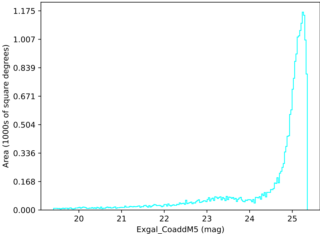
weather_cloudso14v3.4_10yrs All sky u band: Exgal_CoaddM5
