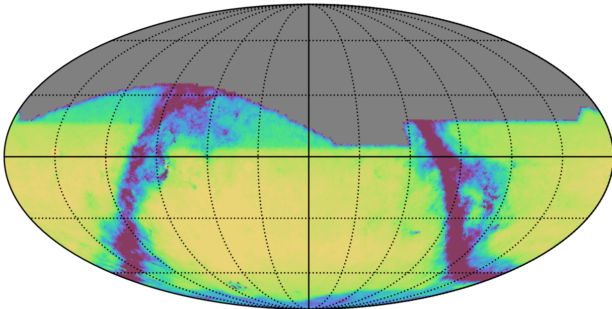
weather_cloudso14v3.4_10yrs All sky r band: Exgal_CoaddM5
