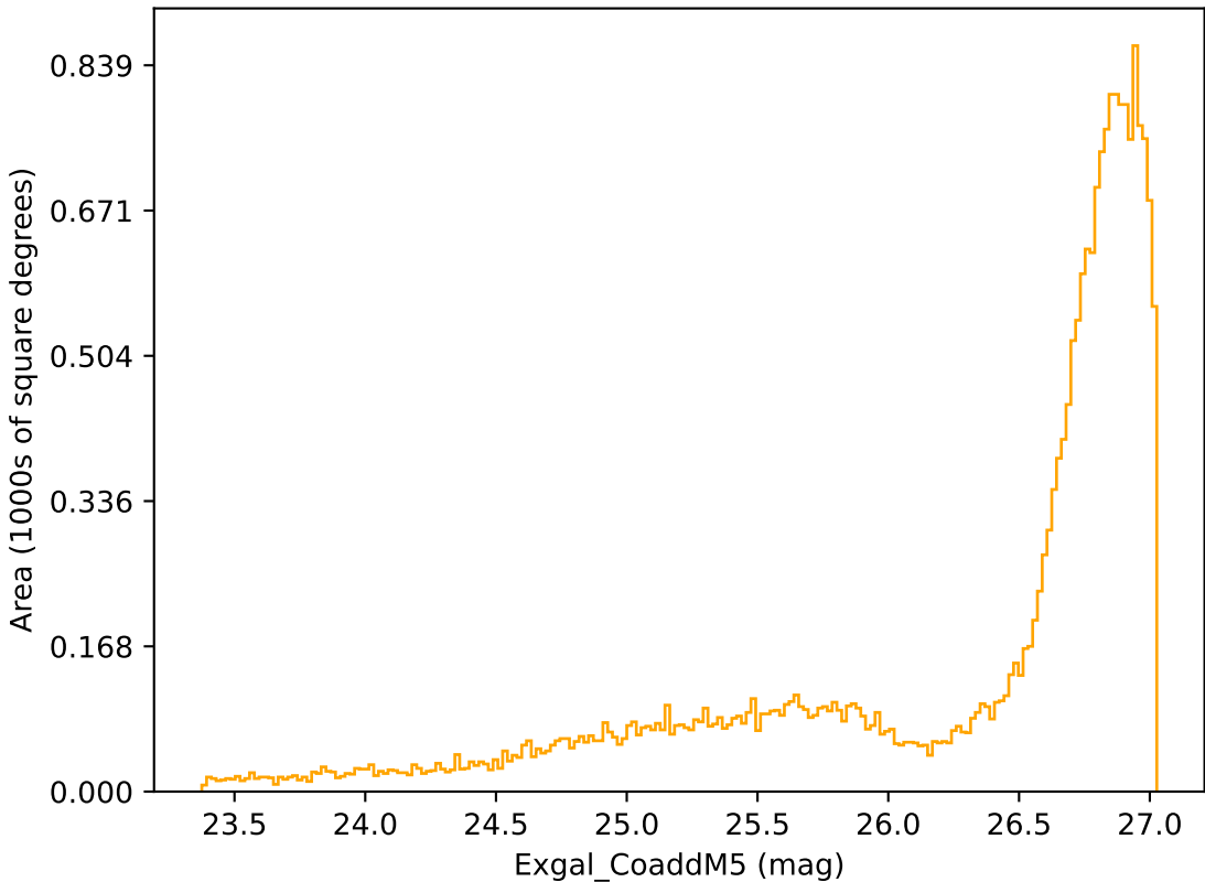
weather_cloudso14v3.4_10yrs All sky r band: Exgal_CoaddM5
