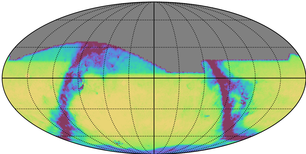
weather_cloudso14v3.4_10yrs All sky i band: Exgal_CoaddM5
