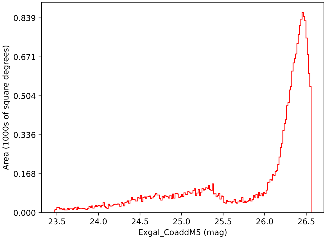
weather_cloudso14v3.4_10yrs All sky i band: Exgal_CoaddM5
