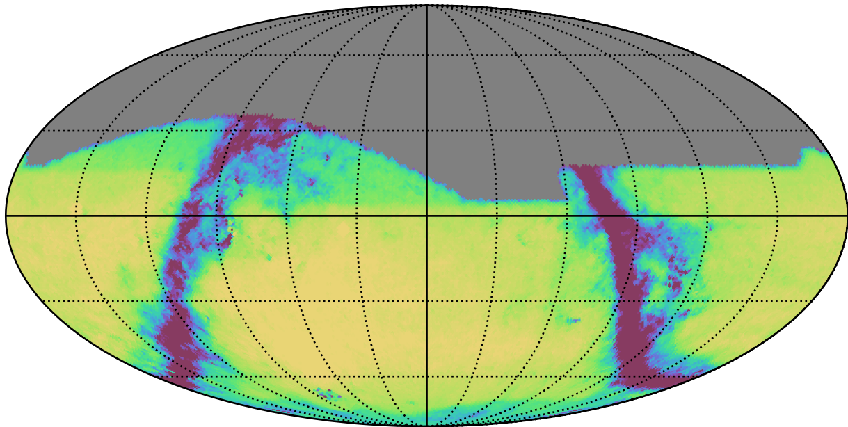
weather_cloudso14v3.4_10yrs All sky g band: Exgal_CoaddM5
