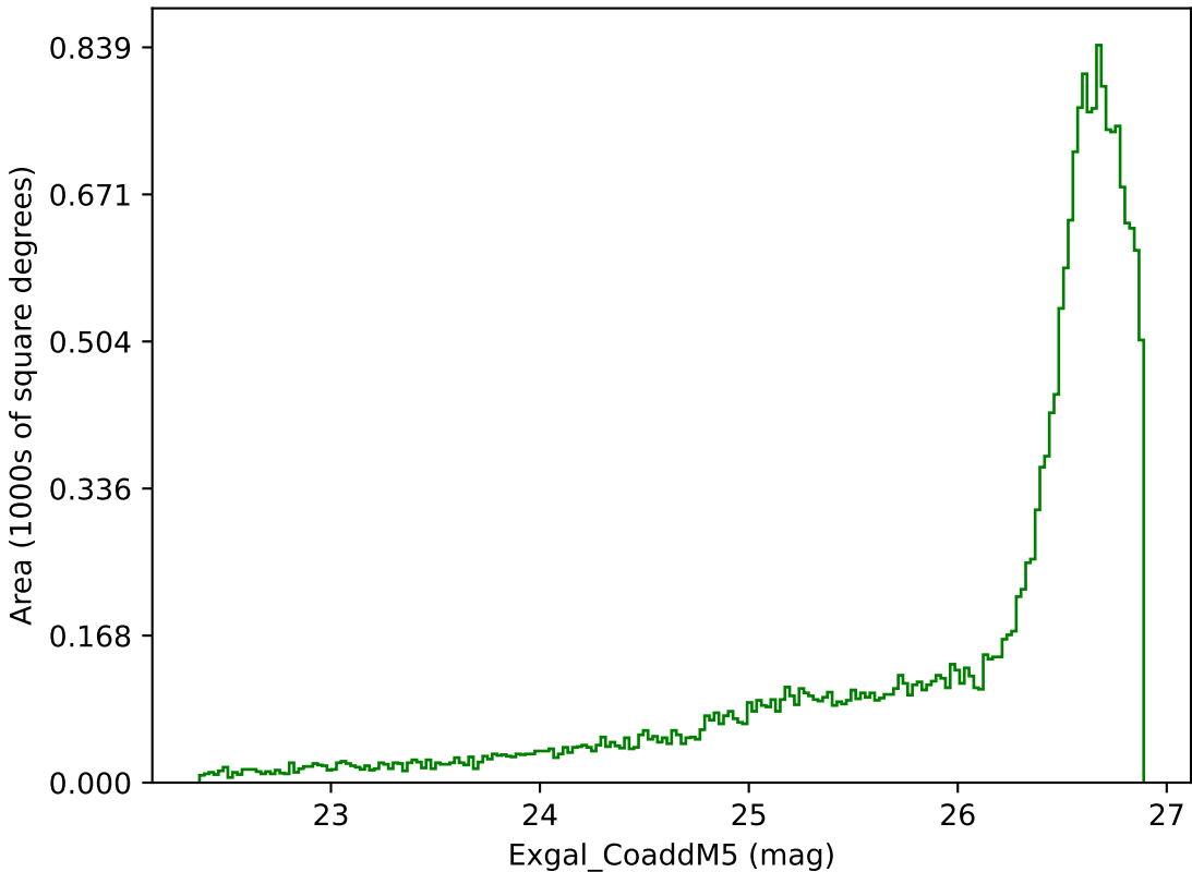
weather_cloudso14v3.4_10yrs All sky g band: Exgal_CoaddM5
