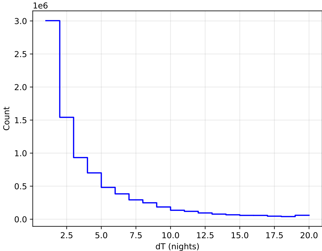
weather_cloudso14v3.4_10yrs WFD all bands: DeltaNight Histogram
