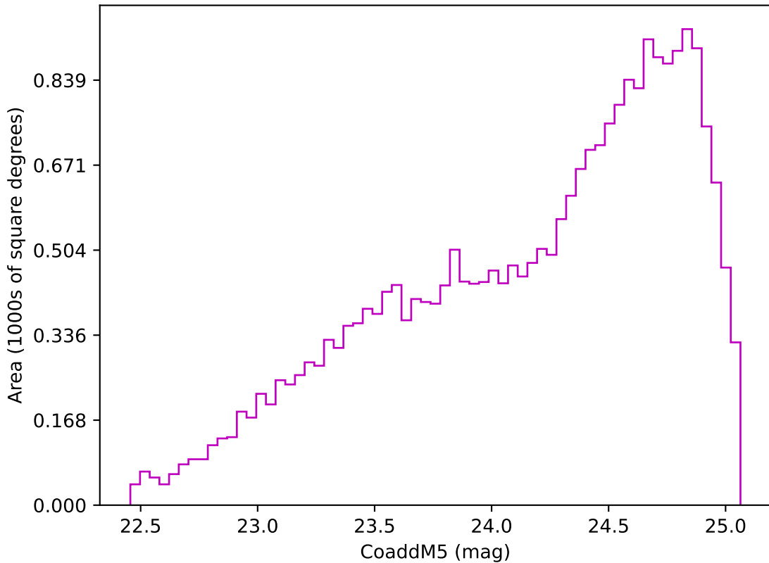
weather_cloudso14v3.4_10yrs Yr 3-4 z band: CoaddM5
