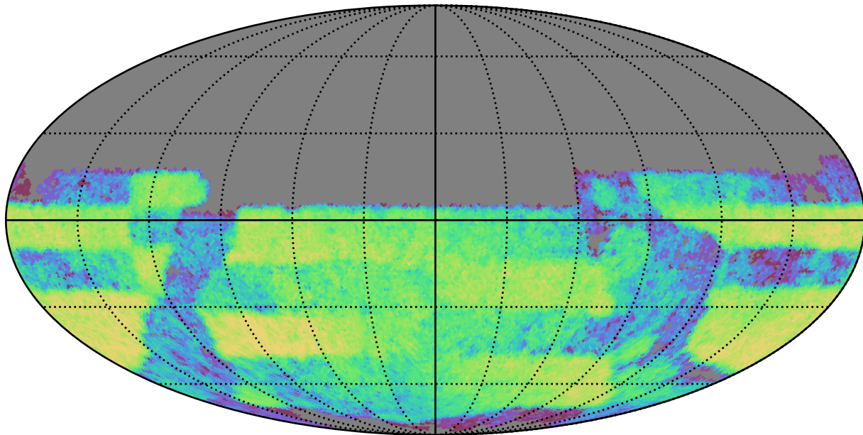
weather_cloudso14v3.4_10yrs Yr 3-4 y band: CoaddM5
