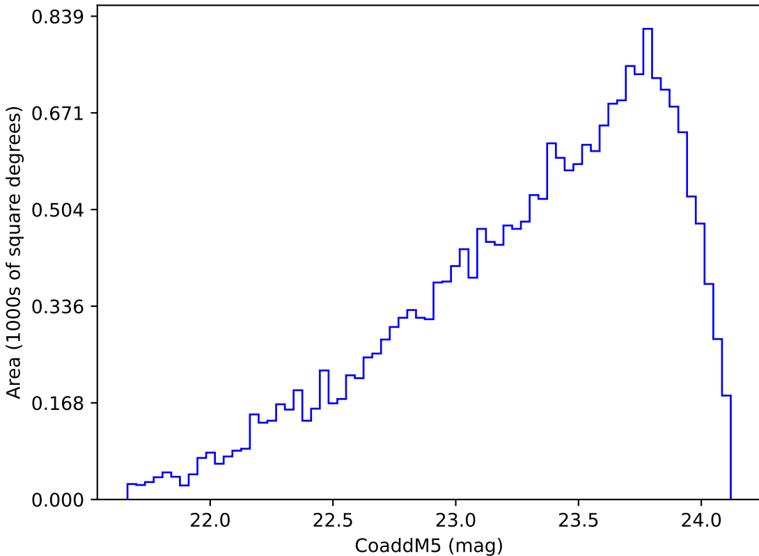
weather_cloudso14v3.4_10yrs Yr 3-4 y band: CoaddM5
