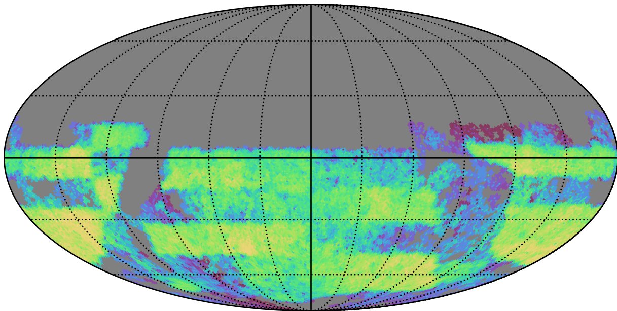
weather_cloudso14v3.4_10yrs Yr 3-4 u band: CoaddM5
