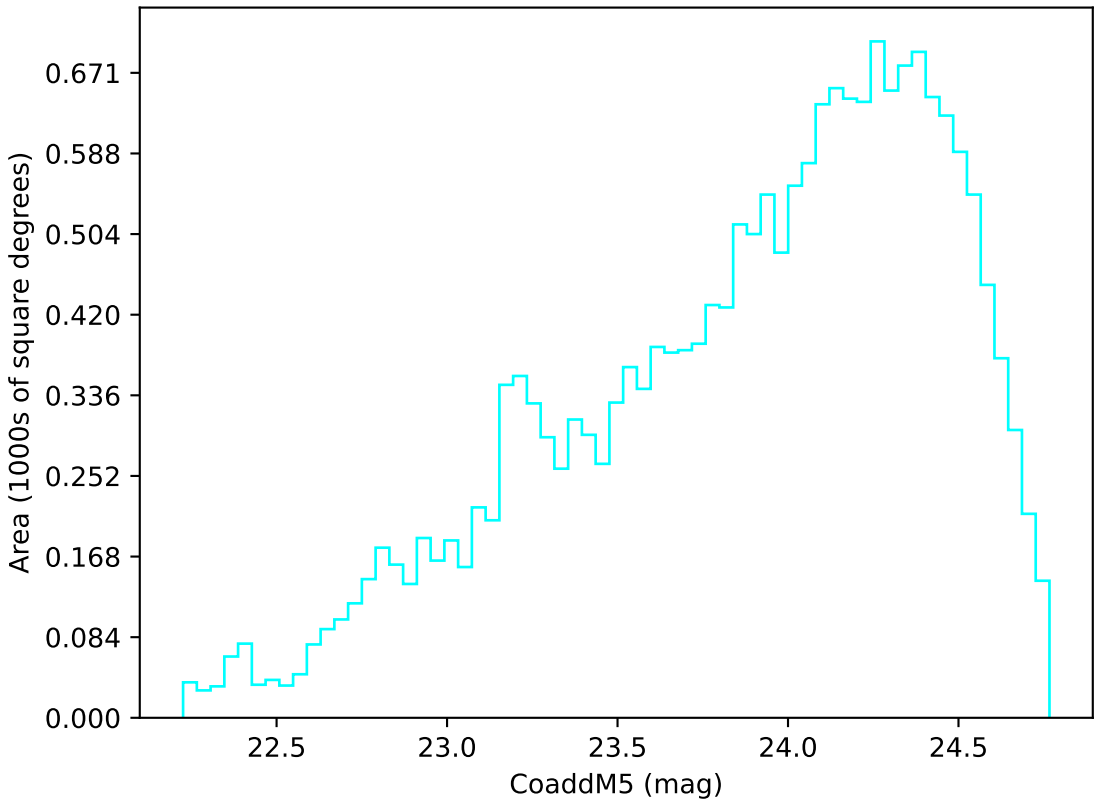
weather_cloudso14v3.4_10yrs Yr 3-4 u band: CoaddM5
