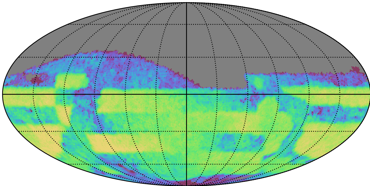
weather_cloudso14v3.4_10yrs Yr 3-4 i band: CoaddM5
