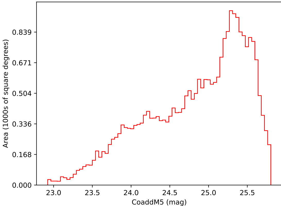
weather_cloudso14v3.4_10yrs Yr 3-4 i band: CoaddM5
