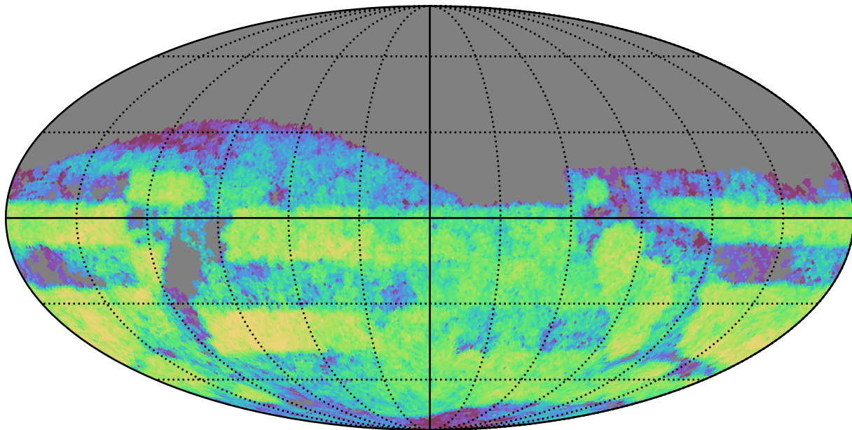
weather_cloudso14v3.4_10yrs Yr 3-4 g band: CoaddM5
