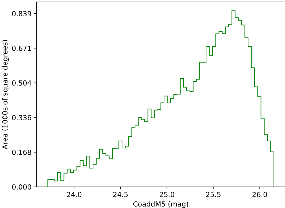
weather_cloudso14v3.4_10yrs Yr 3-4 g band: CoaddM5
