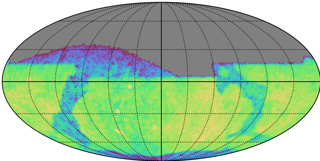
weather_cloudso14v3.4_10yrs Yr 1 z band: CoaddM5
