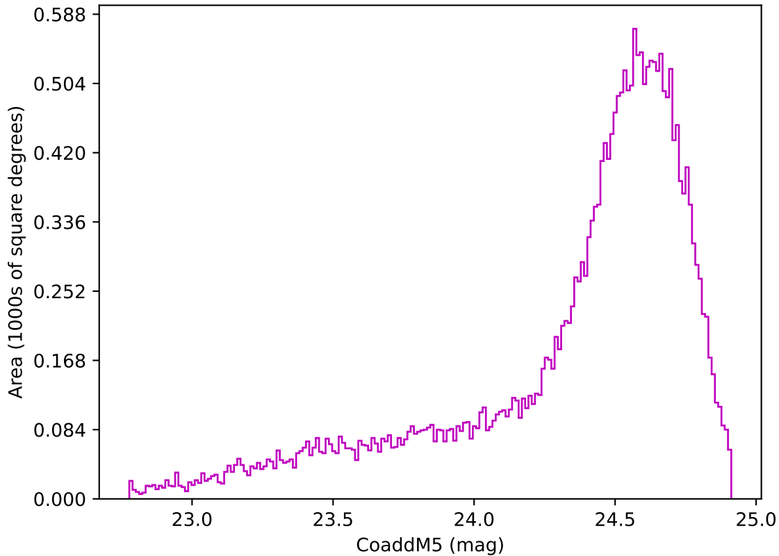
weather_cloudso14v3.4_10yrs Yr 1 z band: CoaddM5
