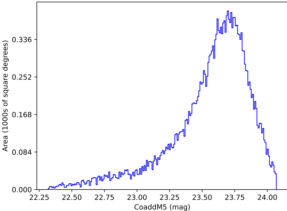
weather_cloudso14v3.4_10yrs Yr 1 y band: CoaddM5
