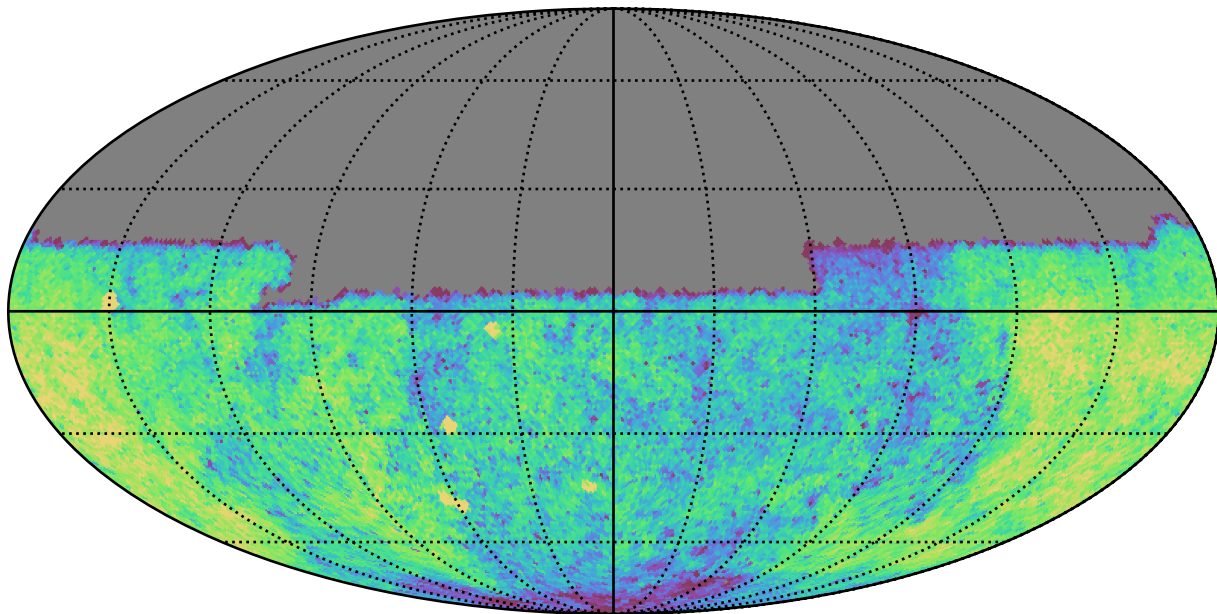
weather_cloudso14v3.4_10yrs Yr 1 u band: CoaddM5
