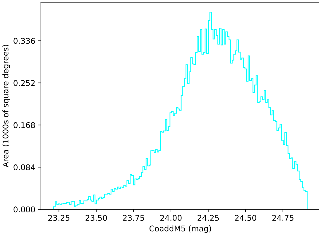
weather_cloudso14v3.4_10yrs Yr 1 u band: CoaddM5
