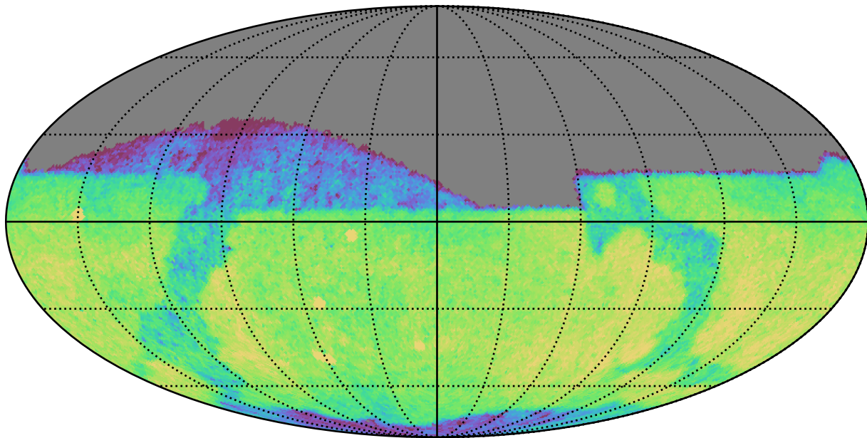
weather_cloudso14v3.4_10yrs Yr 1 r band: CoaddM5
