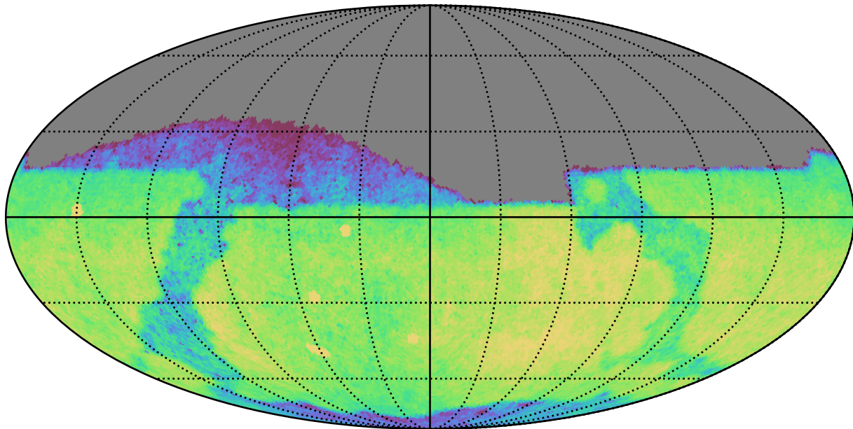
weather_cloudso14v3.4_10yrs Yr 1 i band: CoaddM5
