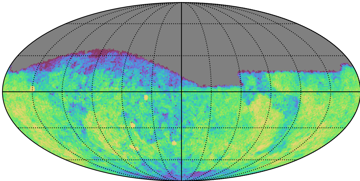
weather_cloudso14v3.4_10yrs Yr 1 g band: CoaddM5
