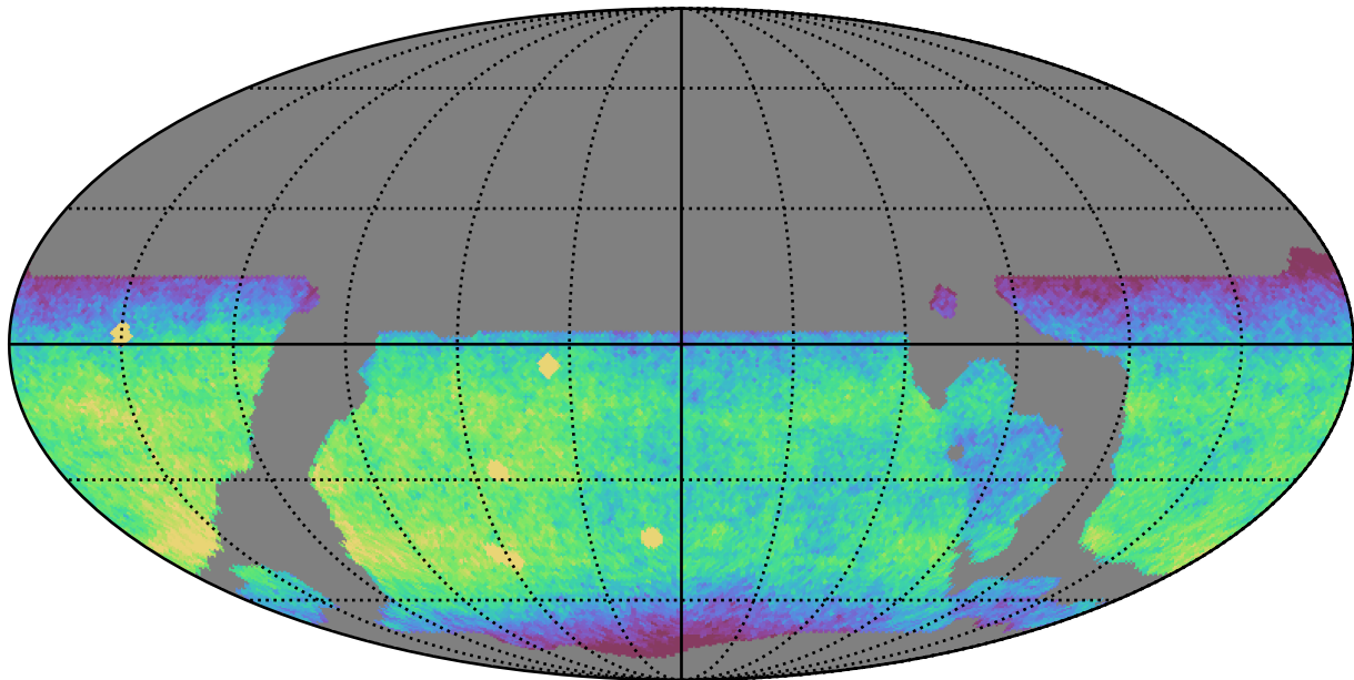
weather_cloudso14v3.4_10yrs WFD z band: CoaddM5
