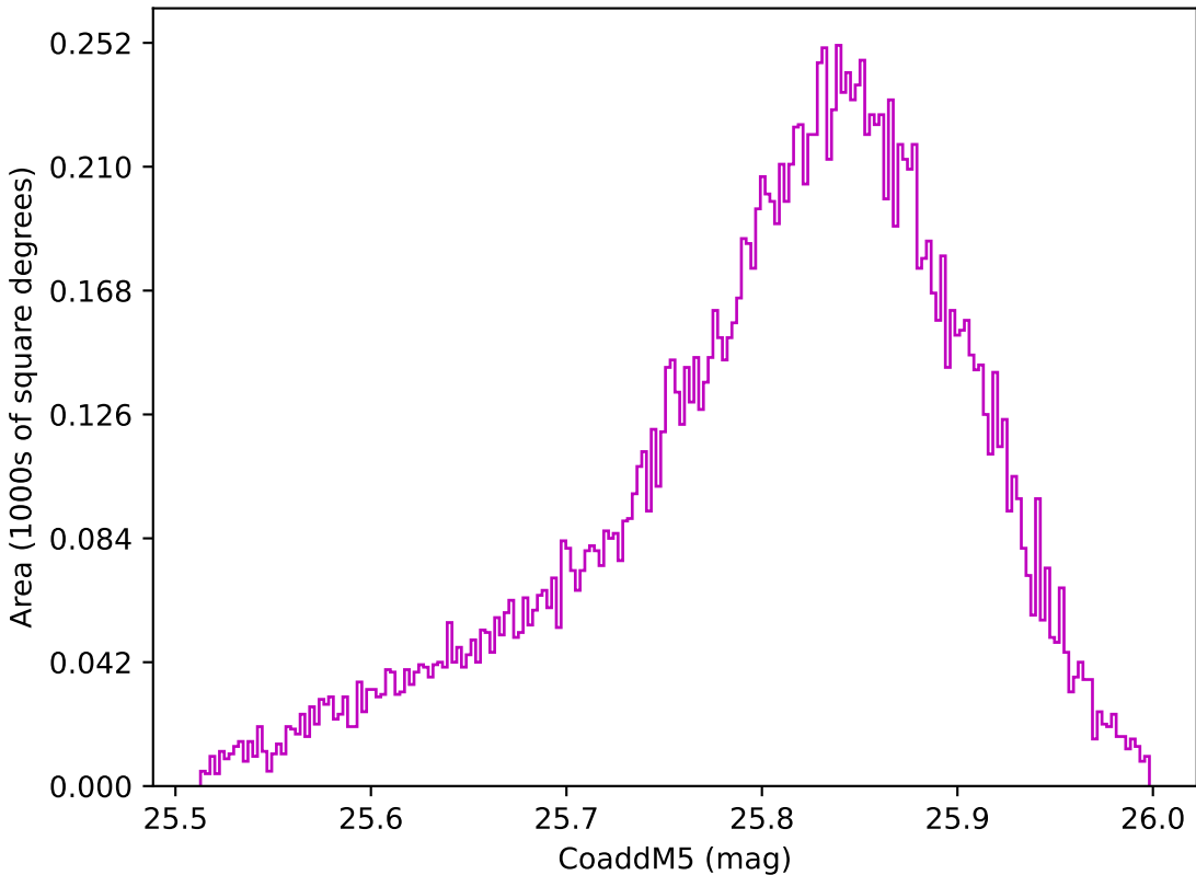
weather_cloudso14v3.4_10yrs WFD z band: CoaddM5
