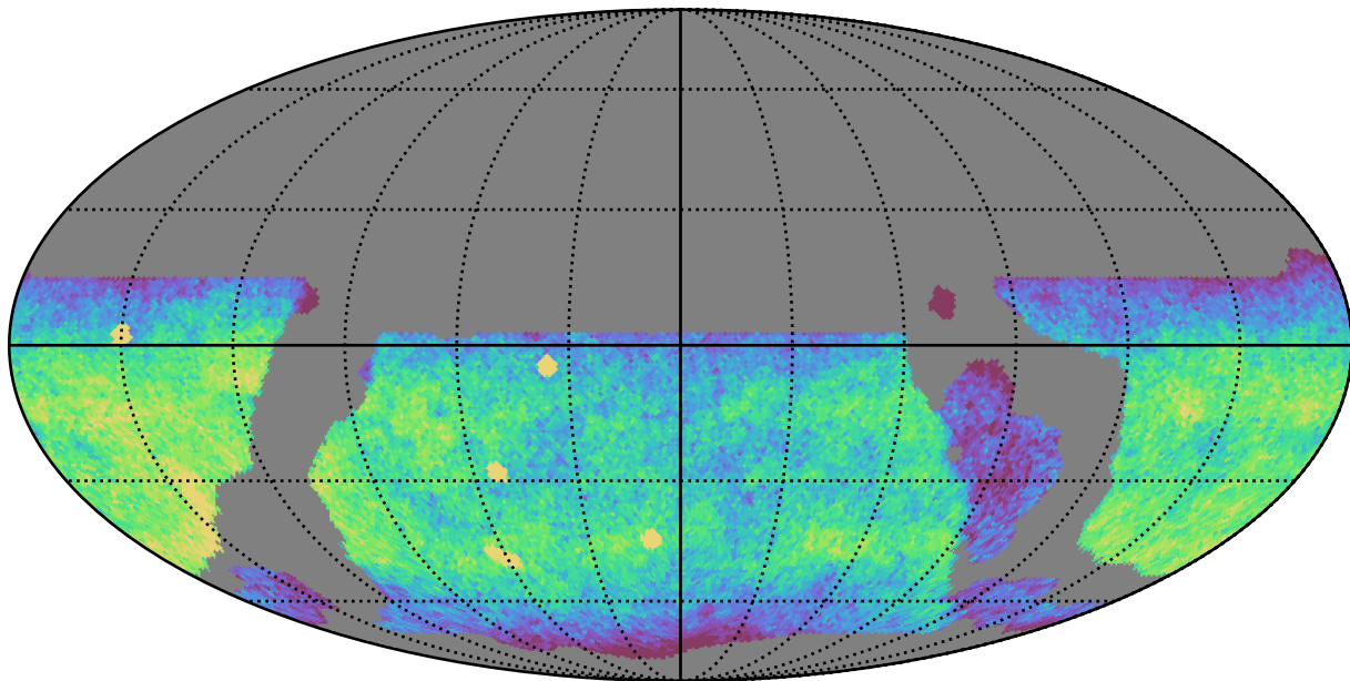
weather_cloudso14v3.4_10yrs WFD u band: CoaddM5
