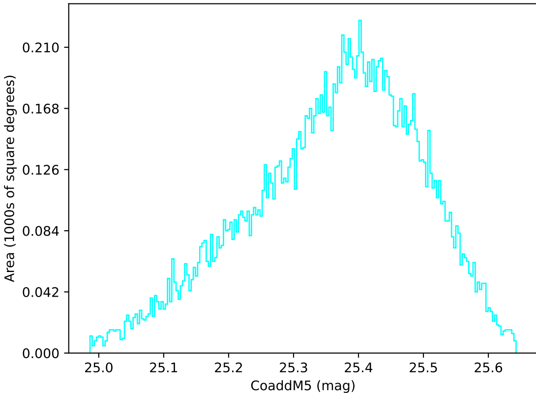
weather_cloudso14v3.4_10yrs WFD u band: CoaddM5
