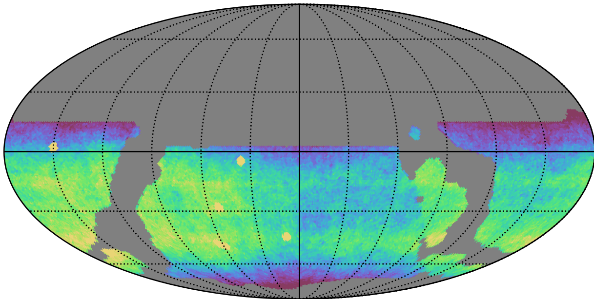
weather_cloudso14v3.4_10yrs WFD r band: CoaddM5
