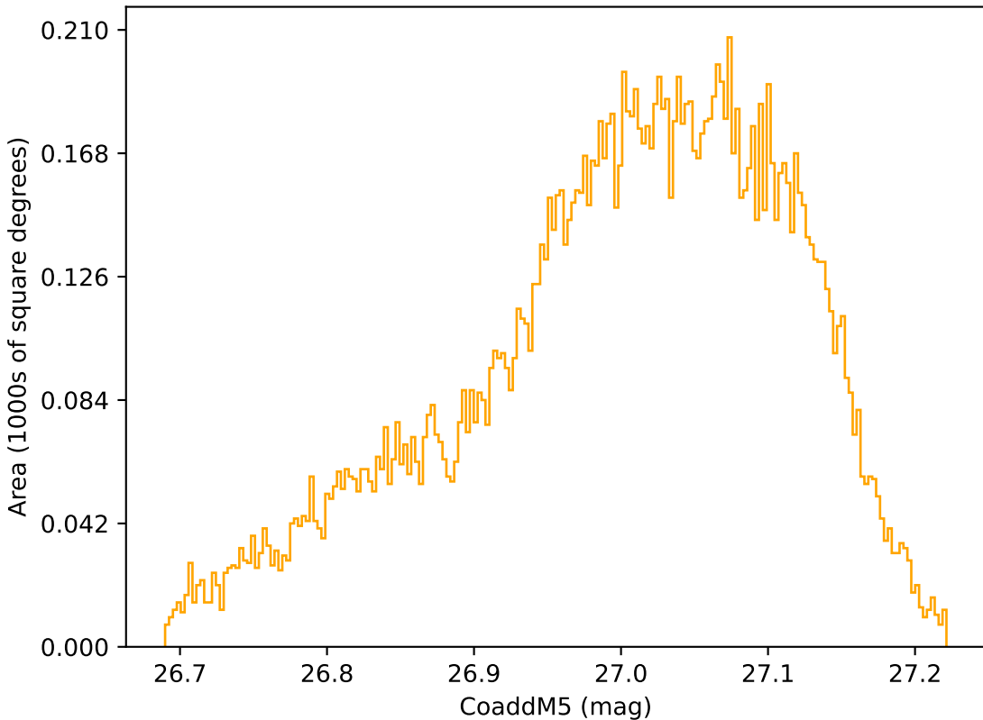
weather_cloudso14v3.4_10yrs WFD r band: CoaddM5
