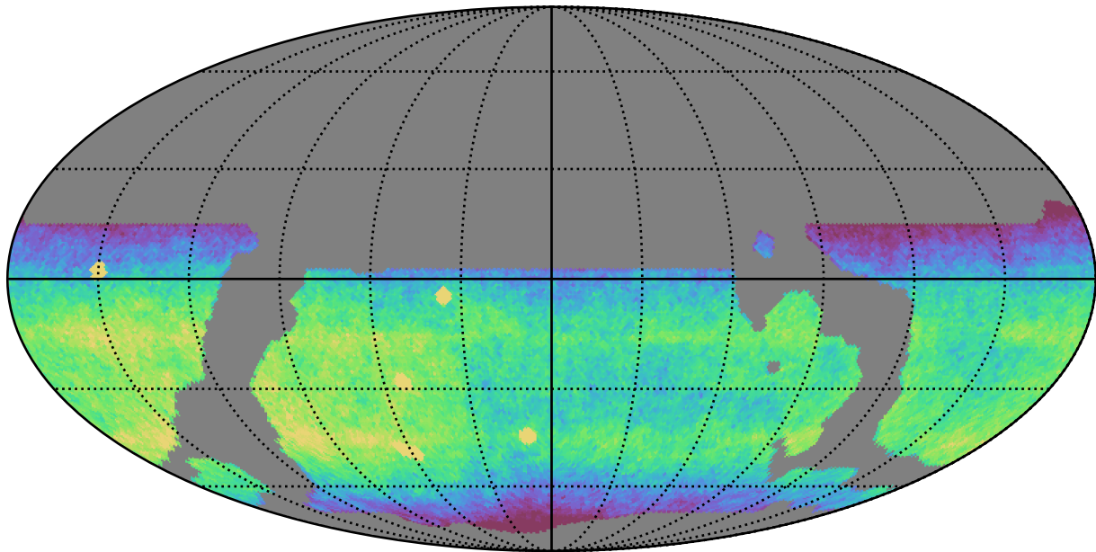
weather_cloudso14v3.4_10yrs WFD i band: CoaddM5
