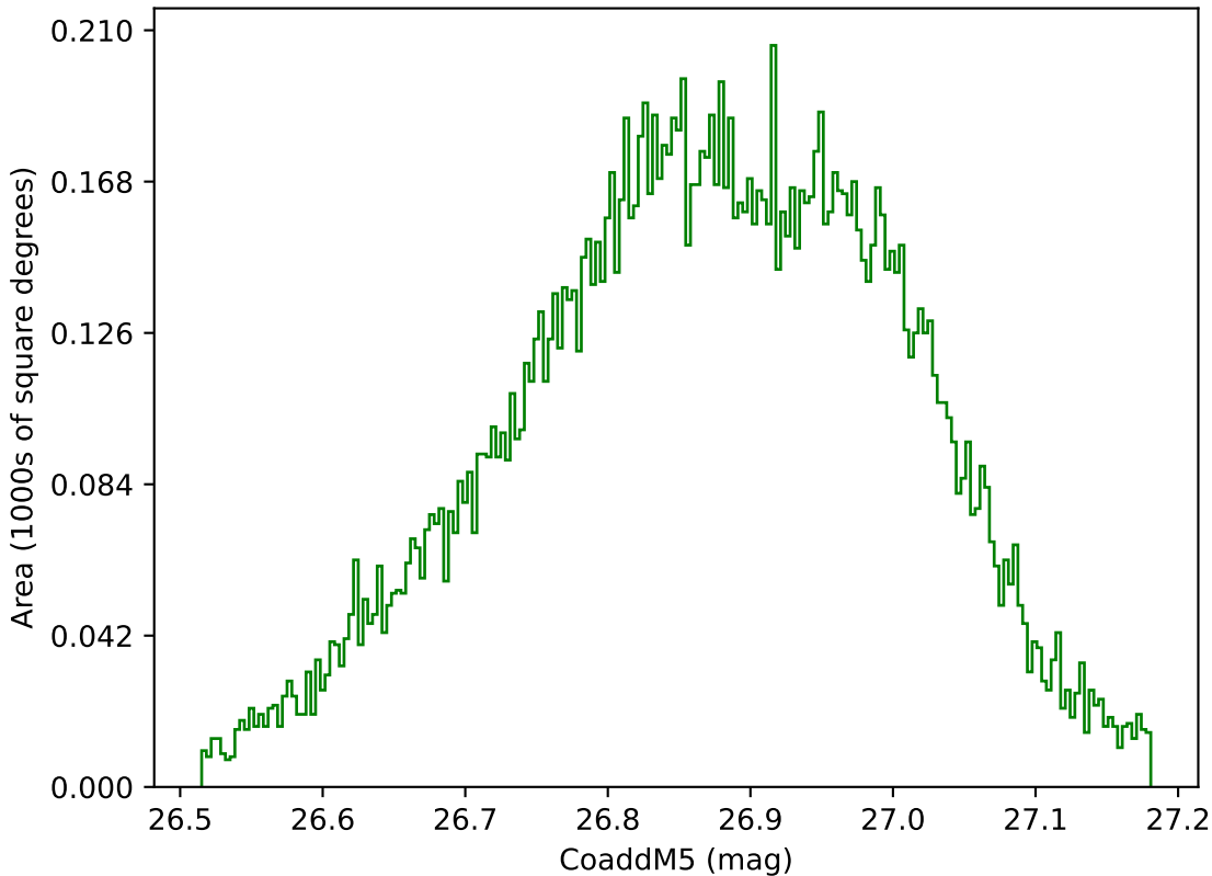
weather_cloudso14v3.4_10yrs WFD g band: CoaddM5
