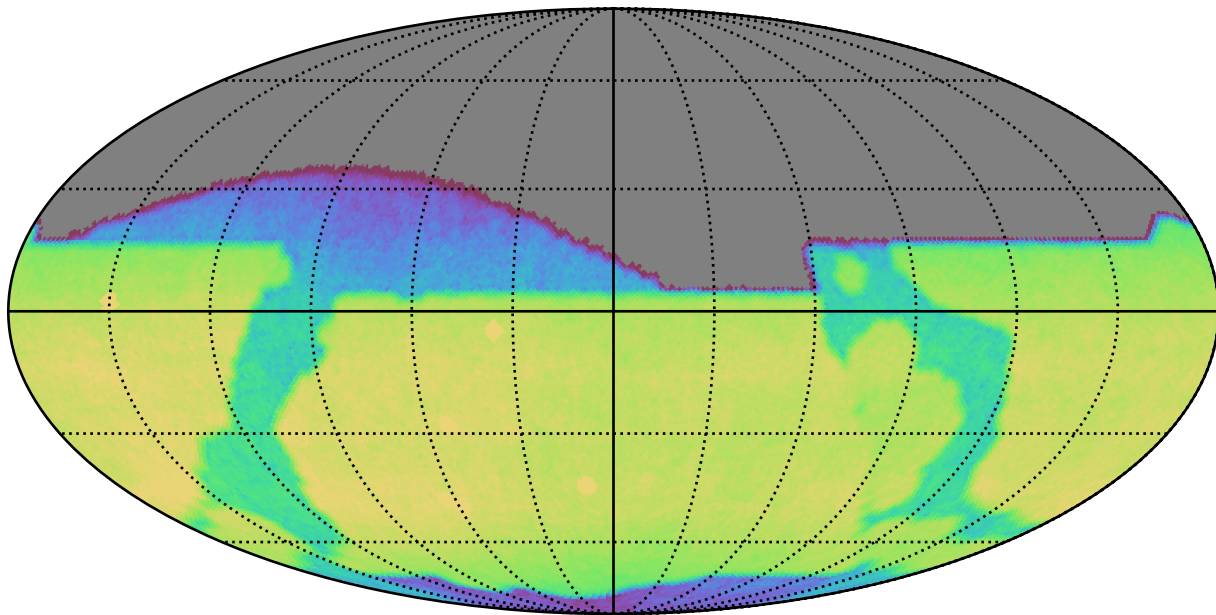
weather_cloudso14v3.4_10yrs All sky z band: CoaddM5
