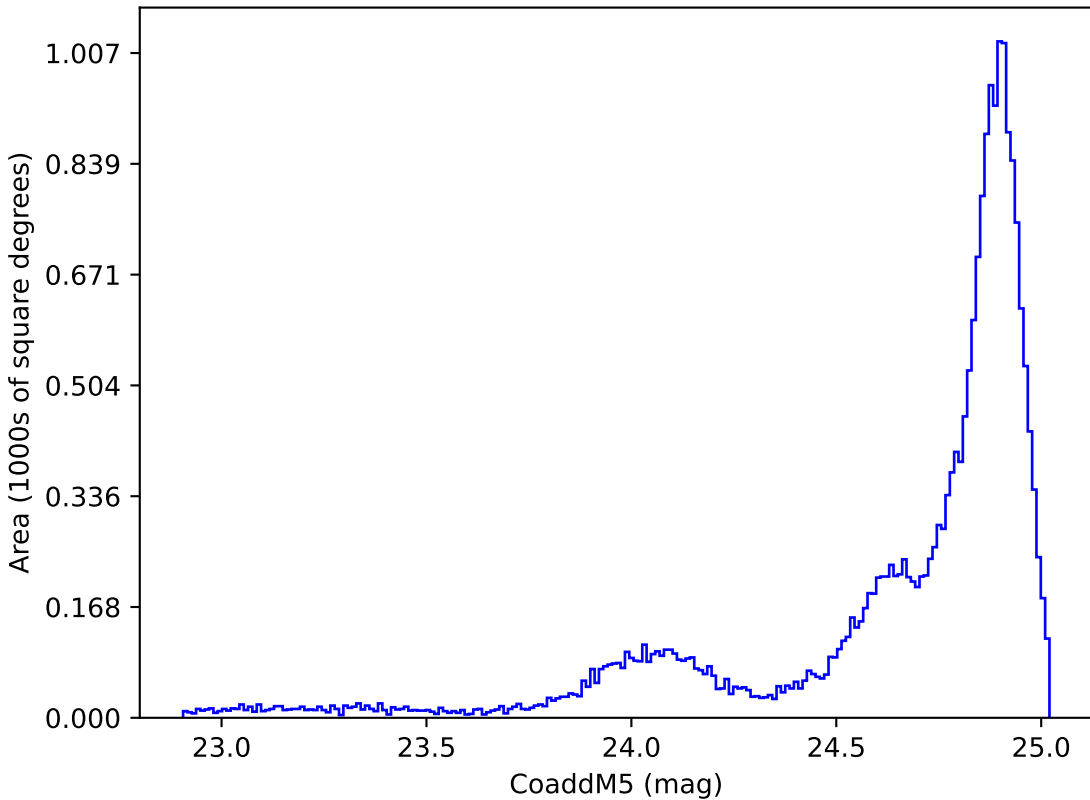
weather_cloudso14v3.4_10yrs All sky y band: CoaddM5
