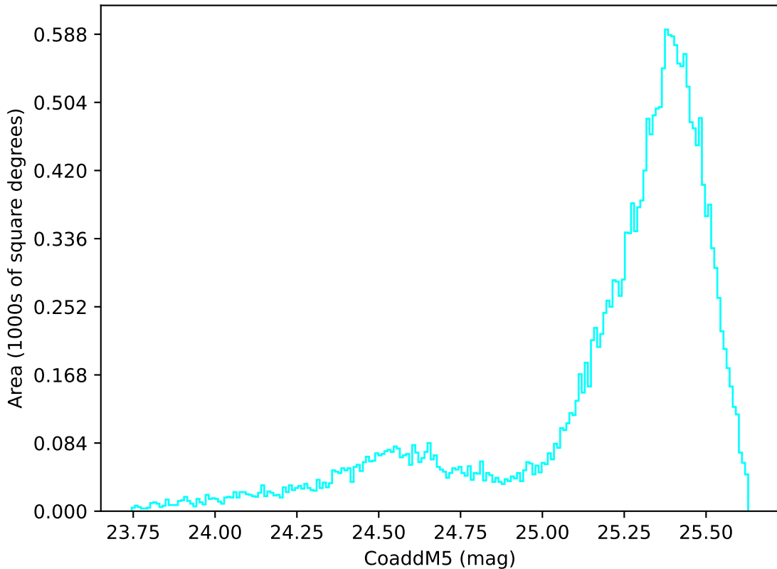
weather_cloudso14v3.4_10yrs All sky u band: CoaddM5
