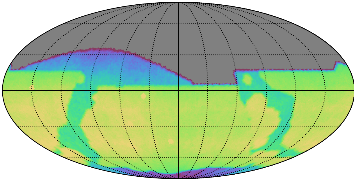
weather_cloudso14v3.4_10yrs All sky r band: CoaddM5
