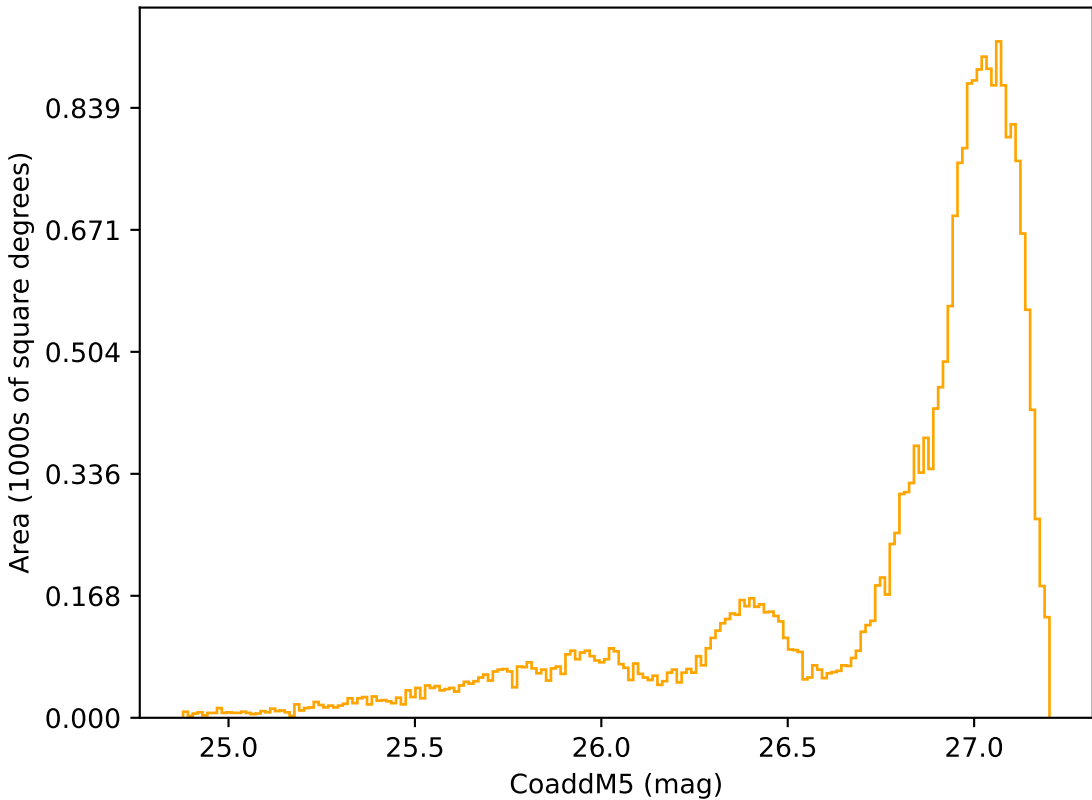
weather_cloudso14v3.4_10yrs All sky r band: CoaddM5
