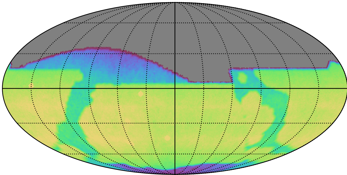
weather_cloudso14v3.4_10yrs All sky i band: CoaddM5
