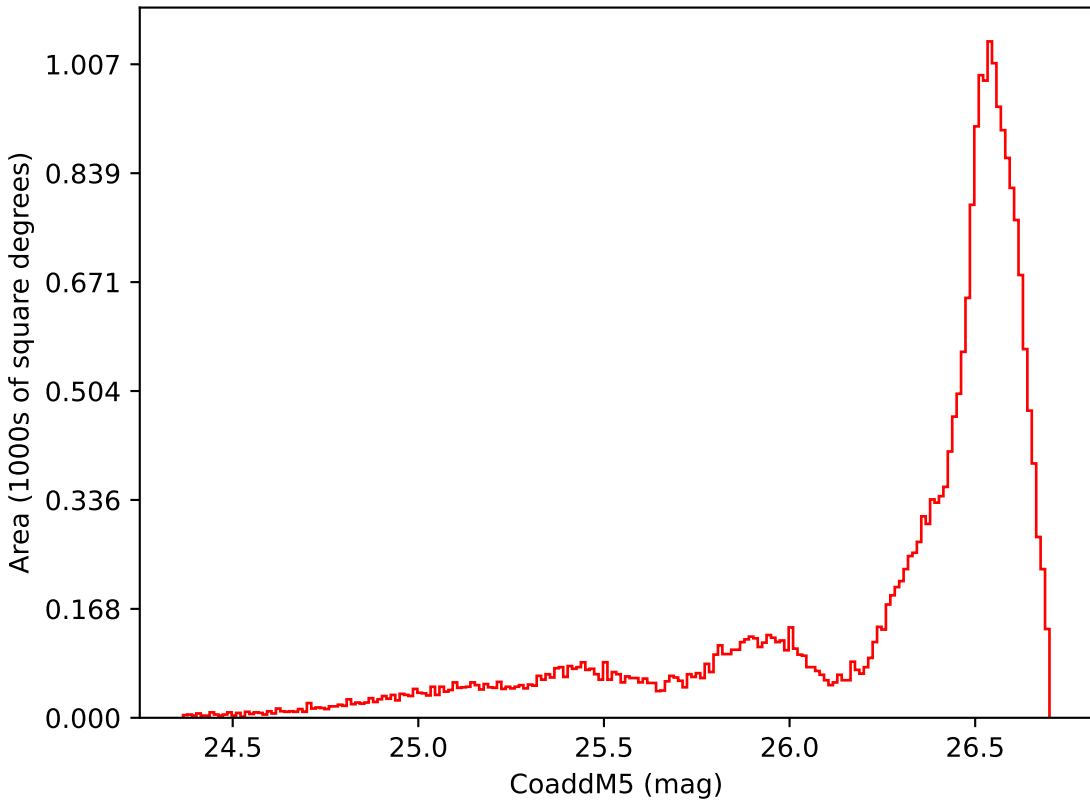
weather_cloudso14v3.4_10yrs All sky i band: CoaddM5
