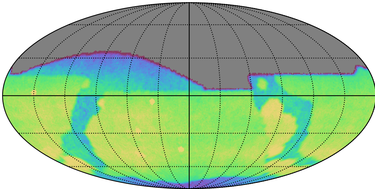
weather_cloudso14v3.4_10yrs All sky g band: CoaddM5
