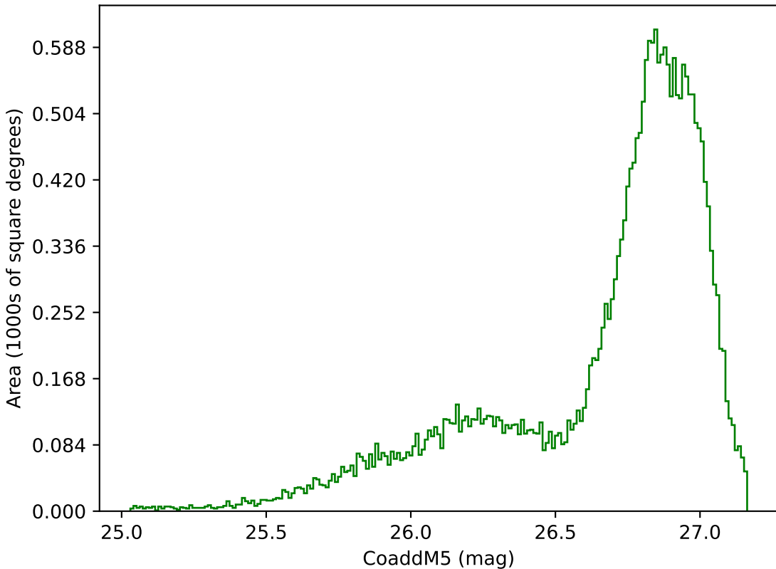
weather_cloudso14v3.4_10yrs All sky g band: CoaddM5
