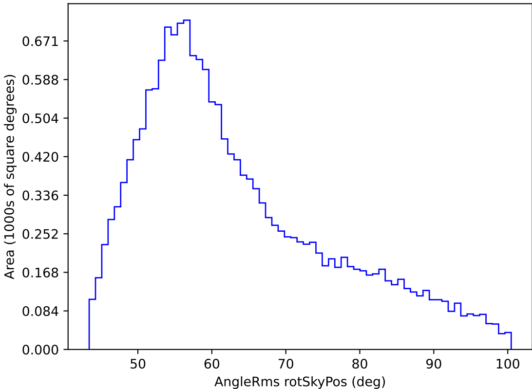
weather_cloudso14v3.4_10yrs WFD u band: AngleRms rotSkyPos
