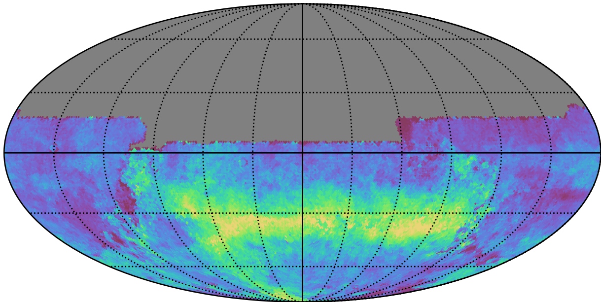
weather_cloudso14v3.4_10yrs All sky u band: AngleRms rotSkyPos
