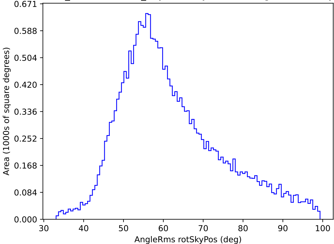
weather_cloudso14v3.4_10yrs All sky u band: AngleRms rotSkyPos
