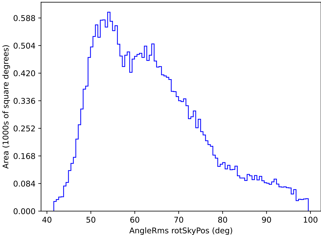
weather_cloudso14v3.4_10yrs All sky r band: AngleRms rotSkyPos
