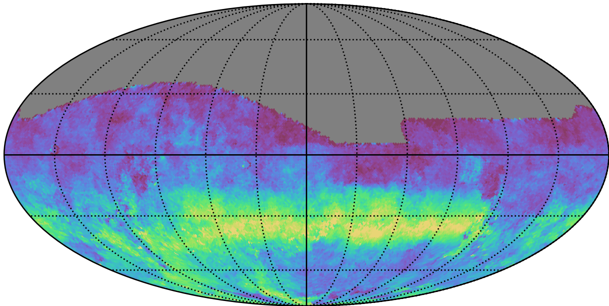
weather_cloudso14v3.4_10yrs All sky g band: AngleRms rotSkyPos
