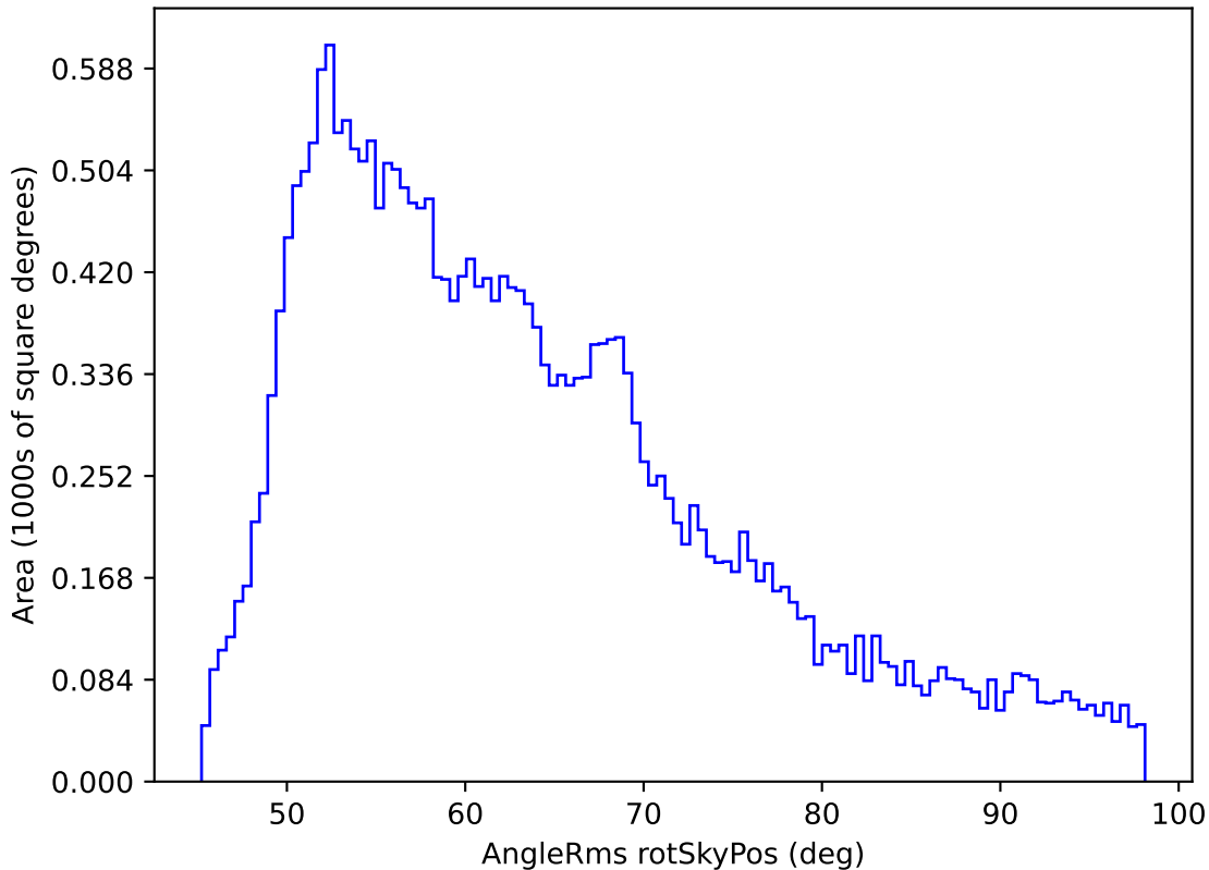
weather_cloudso14v3.4_10yrs All sky all bands: AngleRms rotSkyPos
