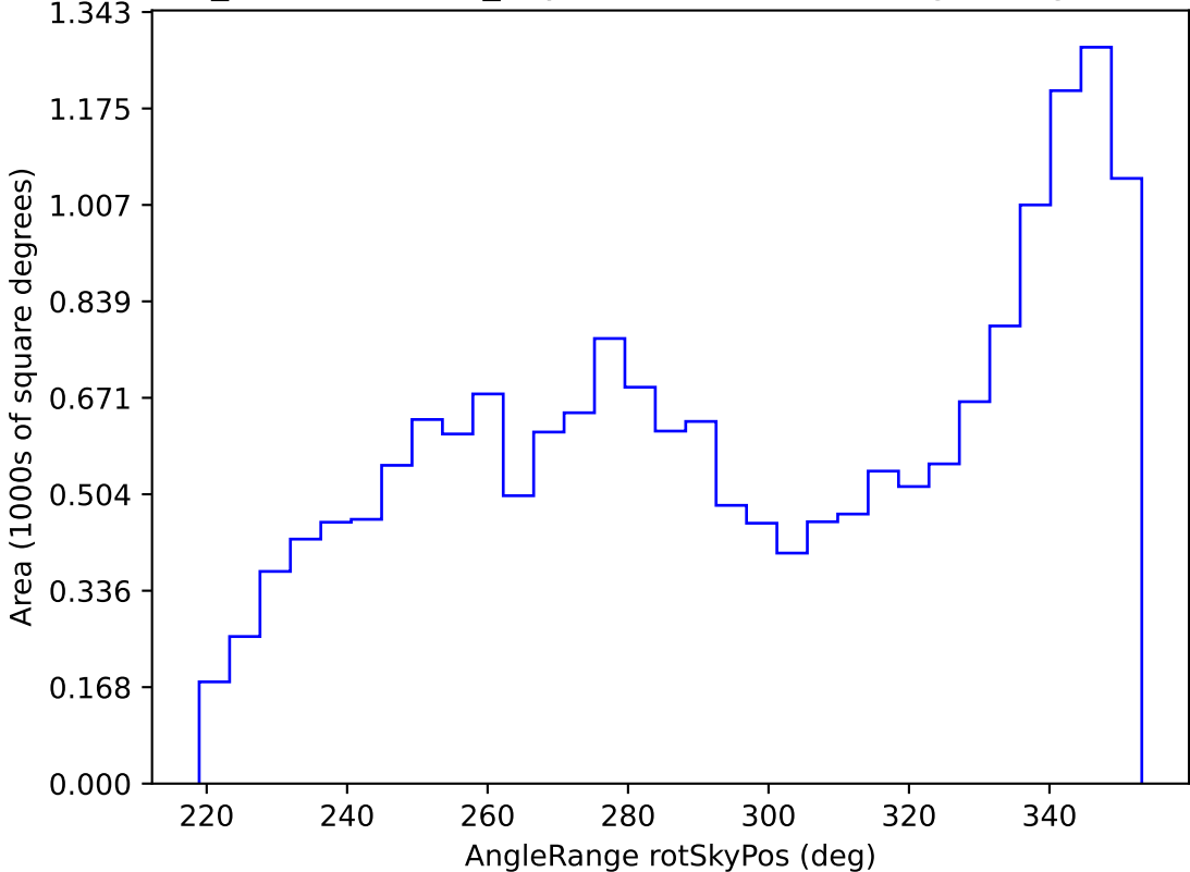
weather_cloudso14v3.4_10yrs WFD all bands: AngleRange rotSkyPos
