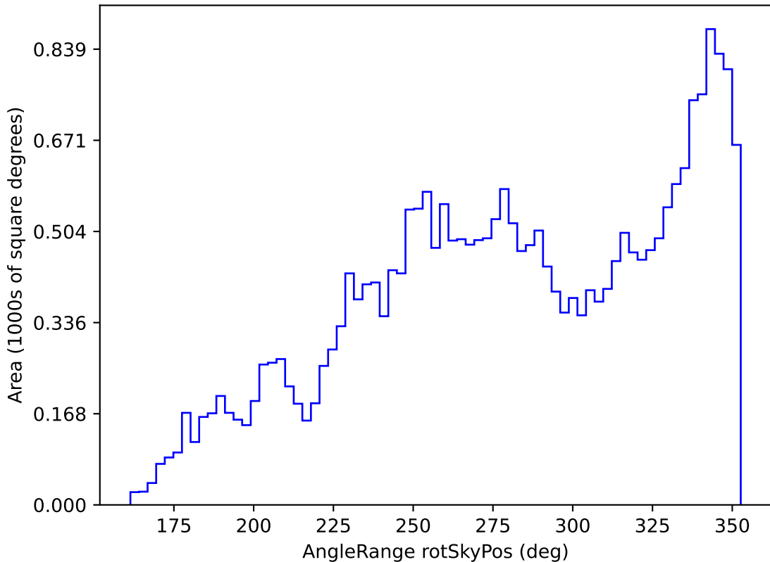
weather_cloudso14v3.4_10yrs All sky all bands: AngleRange rotSkyPos
